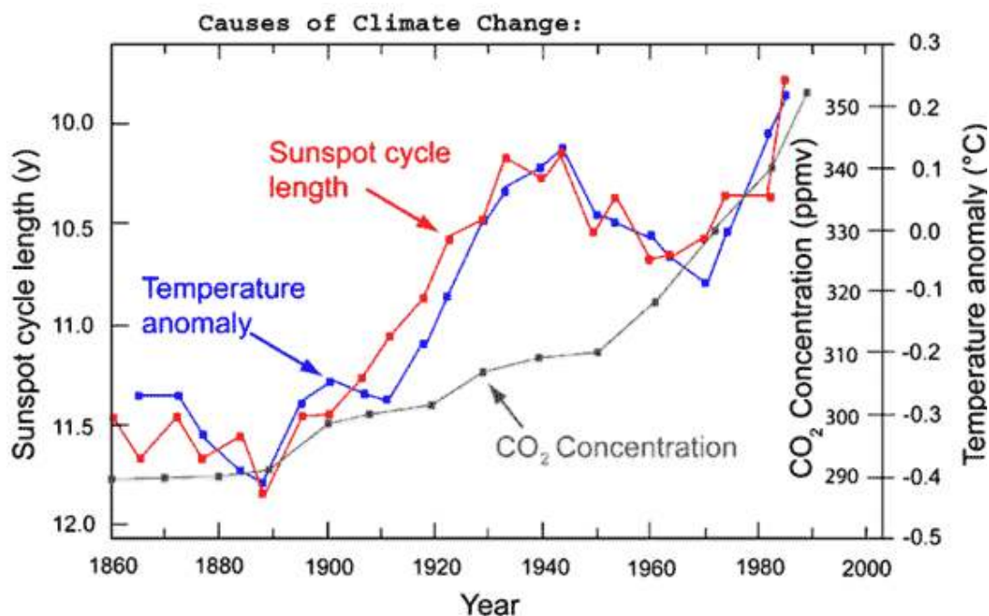
Sunspot cycle length versus smoothed global mean temperatures from 1850 to 1970 and compared with CO 2 concentration
